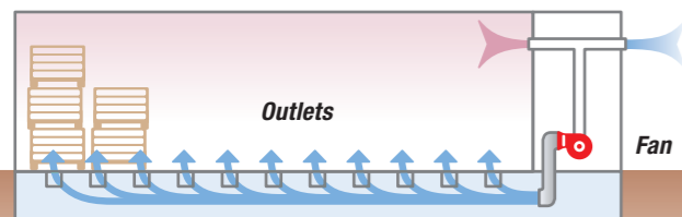
Cross section of a potato warehouse: fans blow fresh air through a duct to the outlets
